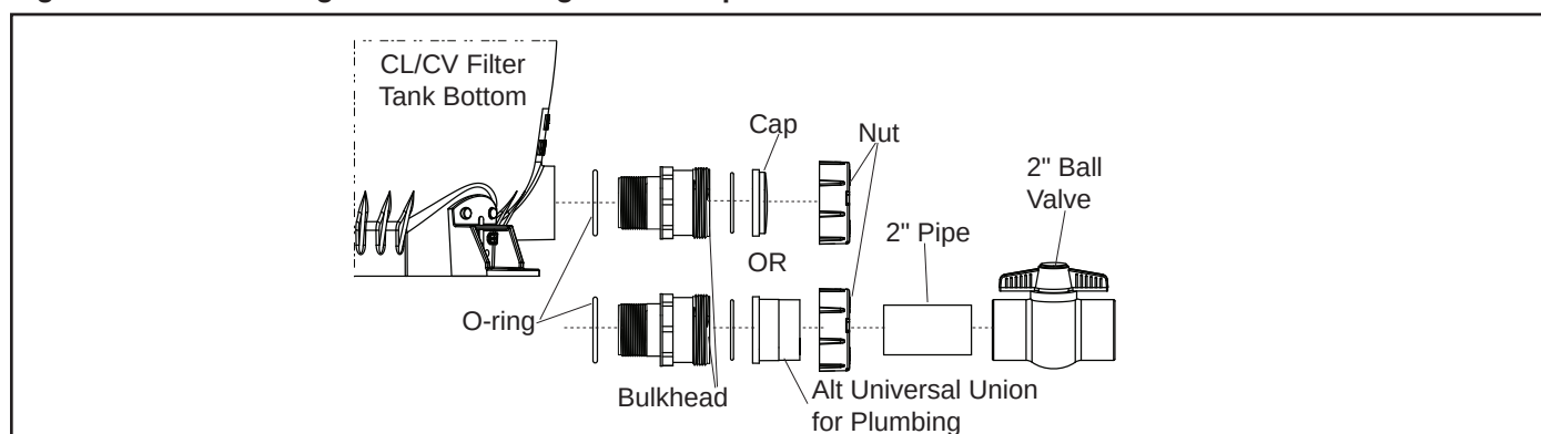
Figure 6. Jandy CL and CV Series Cartridge Filter Drain Configurations
