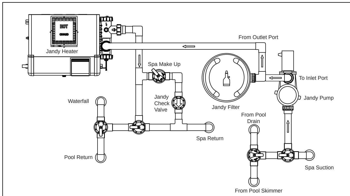
Figure 5. CL Cartridge Filter Plumbing for Pool/Spa Combination
